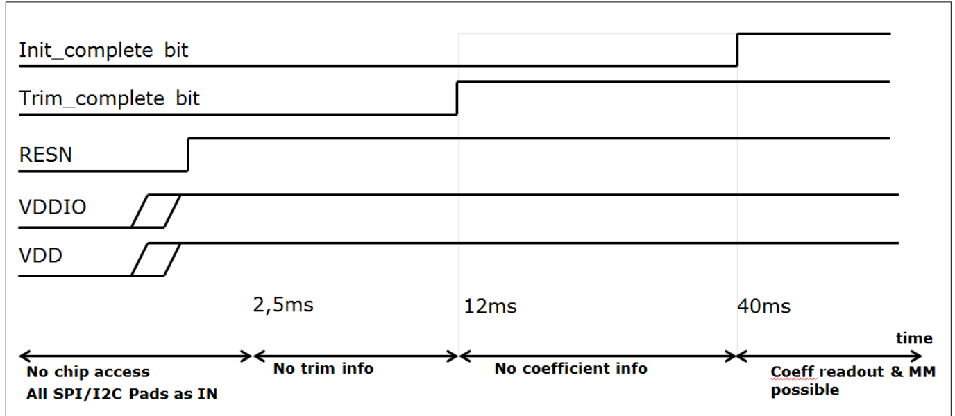
Figure 4 Start-up sequence
