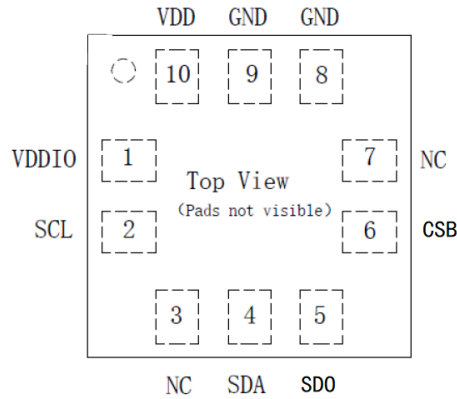
Figure 1 Pin configuration (topview, figure not to scale)
